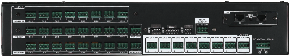
Rear panel
