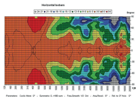
Polar diagrams
