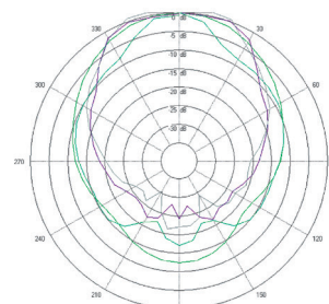
Horizontal directivity
