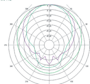
Vertical directivity
