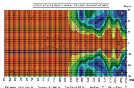
Polar diagrams
