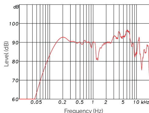
Bandwidth
